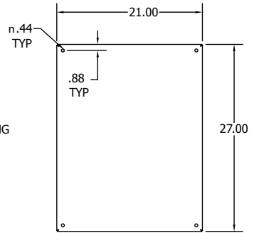
ALUMINUM PANEL
