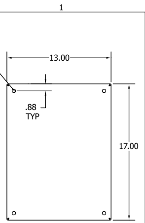
ALUMINUM PANEL
