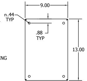
ALUMINUM PANEL
