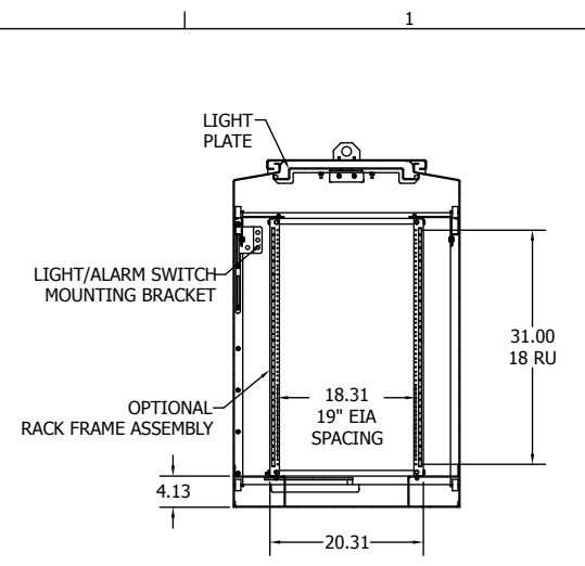
SECTION E-E
