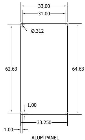
ALUM PANEL
