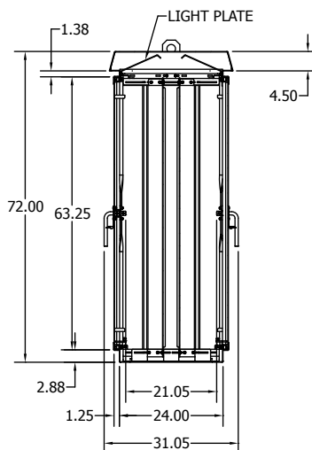
SECTION G-G
