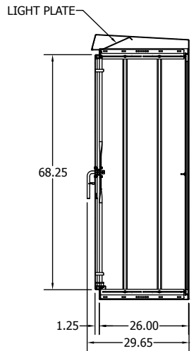
SECTION C-C
