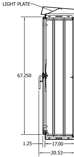
SECTION F-F
