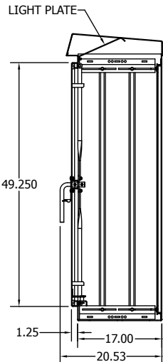
SECTION F-F
