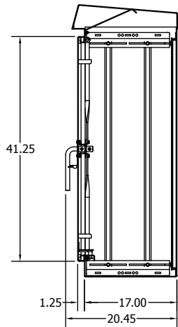
SECTION F-F
