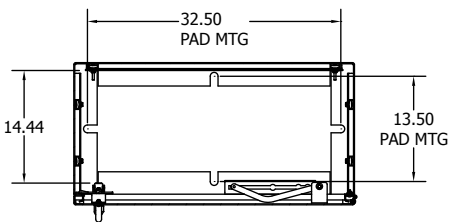
SECTION E-E
